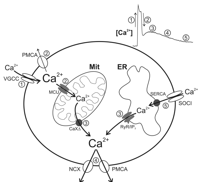
Figure 10. \text{Ca}^{2+} from multiple sources is cleared by distinct sets of \text{Ca}^{2+} removal systems in the bag cell neurons. A conceptual model of \text{Ca}^{2+} dynamics during an afterdischarge based on the current study and prior work by our laboratory and others (Fink et al., 1988; Fisher et al., 1994; Michel and Wayne, 2002; Kachoei et al., 2006; Geiger and Magoski, 2008). Top, right inset, A sample trace of intracellular \text{Ca}^{2+} presumed to reflect afterdischarge dynamics in vivo . Numbers correspond to a series of chronological events depicted in the main illustration: 1 , During the fast phase of the afterdischarge there is a large \text{Ca}^{2+} influx through action potential-evoked voltage-gated \text{Ca}^{2+} channels (VGCC). 2 , This early \text{Ca}^{2+} influx is predominantly removed by rapid mitochondrial uptake, with ancillary assistance from the PMCA. 3 , \text{Ca}^{2+} accumulates in the mitochondria, after which it is slowly extruded into the cytosol through a TPP-sensitive \text{Ca}^{2+} -exchanger. Additionally, second messenger cascades are activated that initiate \text{Ca}^{2+} liberation from the ER through \text{IP}_3 and ryanodine receptors. 4 , The release of \text{Ca}^{2+} from intracellular stores causes a prolonged rise in cytosolic \text{Ca}^{2+} that is removed by the \text{Na}^+/\text{Ca}^{2+} exchanger and the PMCA. 5 , Last, sustained \text{Ca}^{2+} release during the afterdischarge depletes the ER and initiates store-operated \text{Ca}^{2+} influx: a distinct \text{Ca}^{2+} source that is removed by the SERCA into the ER lumen.
