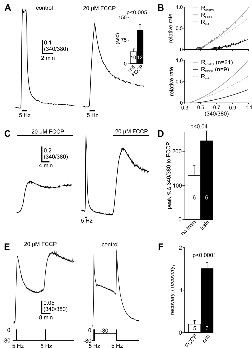
Figure 2. Mitochondria remove voltage-gated \text{Ca}^{2+} influx and clear \text{Ca}^{2+} from repeated stimuli. A , Neurons voltage-clamped to -80 mV with 5 mM intracellular EGTA to allow for isolated measurement of voltage-gated \text{Ca}^{2+} influx and removal. A , Left, In DMSO, cytosolic \text{Ca}^{2+} transients evoked by the 5 Hz, 1 min train stimulus are followed by rapid recovery to baseline \text{Ca}^{2+} . A , Right, Pretreatment with 20 \mu\text{M} FCCP, a protonophore that collapses the mitochondrial membrane potential and prevents \text{Ca}^{2+} sequestration, slows the recovery of \text{Ca}^{2+} following stimulation. A , Inset, The exponential decay time constant ( \tau ) of the \text{Ca}^{2+} transient recovery phase is significantly larger in FCCP-treated neurons (unpaired Student's t test). B , Top, Relative \text{Ca}^{2+} clearance rate ( R ), calculated from the decay phase of \text{Ca}^{2+} transients shown in A , as a function of 340/380 ratio (rates normalized to the maximal value of the 340/380 range). Second-order polynomial fitted lines are plotted overtop of the data points. The difference between the control ( R_{\text{control}} ) and FCCP ( R_{\text{FCCP}} ) fits produce the estimated mitochondrial uptake ( R_{\text{mit}} ), represented by the light dashed line. B , Bottom, Second-order polynomial fit lines for R_{\text{control}} , R_{\text{FCCP}} , and R_{\text{mit}} representing averaged removal rates from multiple neurons. Sample sizes are different from the decay time constants shown in A due to quality of fit criteria required for rate functions (see Materials and Methods). C , \text{Ca}^{2+} influx from a train stimulus loads mitochondria with \text{Ca}^{2+} . C , Left, FCCP (20 \mu\text{M} ) elevates \text{Ca}^{2+} in neurons under voltage clamp at -80 mV with 5 mM EGTA in the pipette and 100 \mu\text{M} TPP to prevent potential release of mitochondrial \text{Ca}^{2+} . C , Right, FCCP-induced \text{Ca}^{2+} release after a large influx of \text{Ca}^{2+} from a 5 Hz, 1 min train stimulus is increased. D , Train stimulation, before FCCP application, significantly enhances the peak percentage change upon FCCP-induced \text{Ca}^{2+} liberation (unpaired Student's t test). E , Mitochondrial \text{Ca}^{2+} clearance is necessary for recovery from repeated stimuli. E , Left, After a train stimulus in FCCP, a second stimulus produces a \text{Ca}^{2+} load that is largely unremoved. E , Right, To replicate the slow \text{Ca}^{2+} recovery in FCCP, a control cell is given a train stimulus, but then subsequently held at -30 mV to allow for a small persistent \text{Ca}^{2+} influx. \text{Ca}^{2+} levels are quickly restored following a second train stimulus when the cell is clamped at -80 mV. F , The ratio between the first and second percentage recovery at 5 min is significantly larger in FCCP-treated neurons (unpaired Student's unpaired t test).
