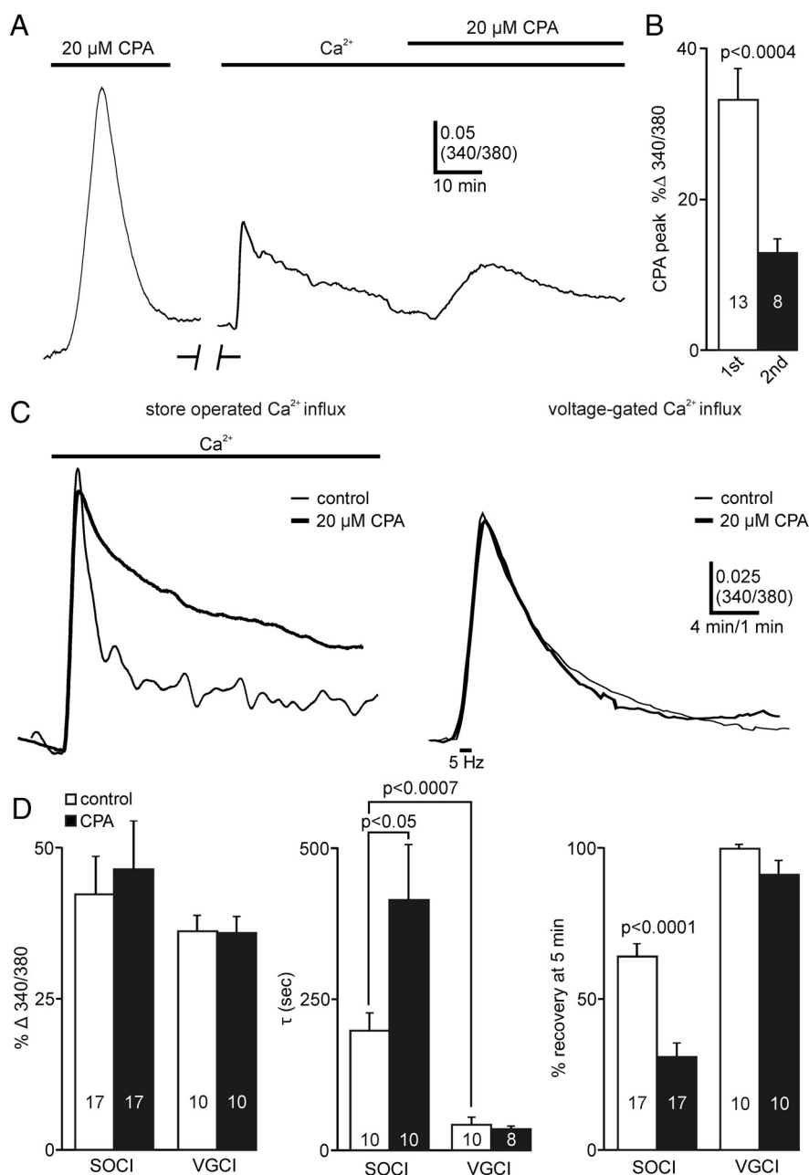
Figure 8. The store-operated \text{Ca}^{2+} influx pathway is cleared by the SERCA to replete the ER. A , Addition of 20 \mu\text{M} CPA depletes ER \text{Ca}^{2+} in a cultured bag cell neuron pressure-injected with fura-PE3. Because neurons are not recorded under voltage clamp, a normal \text{Na}^{+} -containing and \text{K}^{+} -containing external solution is used. After the first depletion, CPA is washed out using bath exchange (at break); upon recording resumption, the addition of extracellular \text{Ca}^{2+} results in a rapid elevation of intracellular \text{Ca}^{2+} . Delivering CPA a second time again evokes a \text{Ca}^{2+} rise, albeit smaller than the first, indicating repletion of the CPA-sensitive store. B , The magnitude of \text{Ca}^{2+} release to the second CPA exposure, after store-operated influx, is significantly smaller than the response elicited during the first CPA-induced depletion (unpaired Student's t test). C , Left, Washout of CPA, before addition of extracellular \text{Ca}^{2+} , speeds the recovery of influx back to baseline. The removal of store-operated \text{Ca}^{2+} recovers at a slower rate in the presence of CPA (dark trace). Both neurons previously depleted in \text{Ca}^{2+} -free ASW with 20 \mu\text{M} CPA. C , Right, \text{Ca}^{2+} influx, similar in size to that evoked by store-operated influx, caused by a short 5 Hz train of depolarizing stimuli from -80 to 0 mV in the presence (dark trace) and absence (light trace) of CPA. CPA has no effect on the speed of recovery from the short stimulus. D , Left, Mean percentage change in 340/380 (left) indicates that the increase in cytosolic \text{Ca}^{2+} during store-operated \text{Ca}^{2+} influx and the short train stimulus \text{Ca}^{2+} influx are not significantly different within and between conditions (ANOVA). D , Middle, CPA significantly increases the mean store-operated \text{Ca}^{2+} influx decay time constant (Welch corrected unpaired Student's t test) although having no effect on the mean \tau of the similarly sized train stimulus-induced \text{Ca}^{2+} influx (unpaired Student's t test). D , Right, The percentage recovery at 5 min (right) after the application of extracellular \text{Ca}^{2+} is significantly shorter with prior CPA washout (Welch corrected unpaired Student's t test). However, the percentage recovery at 5 min after the short train stimulus \text{Ca}^{2+} influx is not significantly altered by CPA.
