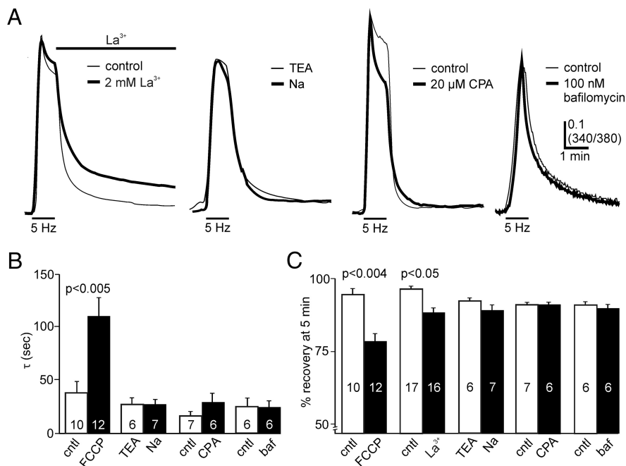
Figure 3. Removal of voltage-gated \text{Ca}^{2+} influx is slowed by inhibition of the PMCA, but is not influenced by acidic stores, ER, or the \text{Na}^+/\text{Ca}^{2+} -exchanger. A , Left, Blocking PMCA function by the addition of 2 mM extracellular \text{La}^{3+} on the last pulse of the 1 min, 5 Hz train stimulus, hinders \text{Ca}^{2+} removal (dark trace), whereas \text{H}_2\text{O} (control) (light trace) applied in the same manner has no effect. A , Middle left, In contrast, the inclusion of \text{Na}^+ (dark trace) rather than TEA (light trace) in the extracellular saline, to permit \text{Na}^+/\text{Ca}^{2+} exchanger activity, has no effect. Similarly, treatment with 20 \mu\text{M} CPA (middle right), to inhibit SERCA, or 100 nM bafilomycin A (baf) (right), to prevent uptake by acidic stores, does not alter \text{Ca}^{2+} removal after a train stimulus. B , Neurons treated with 20 \mu\text{M} FCCP present significantly larger exponential decay time constants ( \tau ) relative to controls (reproduced from Fig. 2A), whereas cells in the presence of extracellular \text{Na}^+ , exposed to CPA, or baf do not have significantly different \tau values (all comparisons using unpaired Student's t test). C , FCCP (Mann–Whitney U test) and \text{La}^{3+} significantly (Welch corrected unpaired Student's t test) reduce the percentage recovery at 5 min post-train stimulus whereas extracellular \text{Na}^+ , CPA, and baf have no effect (all comparisons using unpaired Student's t test).
