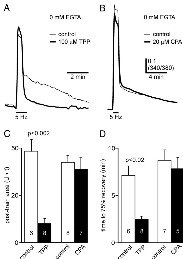
Figure 5. The EGTA-sensitive \text{Ca}^{2+} plateau is caused by mitochondrial \text{Ca}^{2+} release. A , A post-stimulus \text{Ca}^{2+} plateau is evoked by a 5 Hz, 1 min train of depolarizing steps under voltage clamp. Intracellular EGTA is absent (0 mM) to allow for CICR. The prolonged \text{Ca}^{2+} plateau in control conditions (light trace) is substantially smaller in 100 \mu\text{M} the mitochondrial \text{Ca}^{2+} exchange blocker, TPP (dark trace). B , Treatment with CPA, to inhibit SERCA and prevent ER \text{Ca}^{2+} release, does not affect the post-train stimulus \text{Ca}^{2+} plateau (dark trace) when compared with DMSO-treated neurons (light trace). C , D , TPP but not CPA, significantly reduces the 1–11 min area relative to controls (unpaired Student's t test in both cases). TPP also significantly reduces the time to reach 75% recovery of baseline \text{Ca}^{2+} from peak CICR (Welch corrected, unpaired Student's t test). In contrast, CPA has no significant effect on the recovery time (unpaired Student's t test). Sample sizes for the time to 75% recovery in CPA are smaller than those used for post-stimulus area measurements as some neurons did not achieve 75% recovery.
