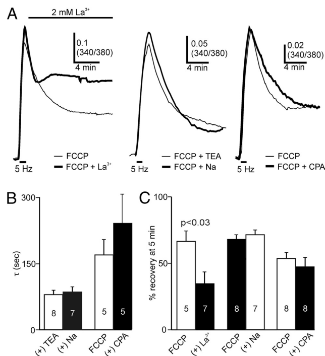
Figure 4. In the absence of mitochondrial function, PMCA, but neither SERCA nor the \text{Na}^+/\text{Ca}^{2+} -exchanger, influence the removal of voltage-gated \text{Ca}^{2+} influx. A , Left, Post-stimulus addition of the PMCA inhibitor, \text{La}^{3+} (2 mM) (dark trace), in the presence of 20 \mu\text{M} FCCP, strongly attenuates the subsequent recovery relative to FCCP alone (light trace). The inclusion of extracellular \text{Na}^+ (middle) or pretreatment with 20 \mu\text{M} CPA (right) does not influence \text{Ca}^{2+} removal in the presence of FCCP. B , For neurons pretreated with FCCP, the mean post-train stimulus recovery \tau values are not significantly altered by the inclusion of extracellular \text{Na}^+ or exposure to CPA (unpaired Student's t test and Mann–Whitney U test, respectively). C , Summary of mean percentage recovery at 5 min post-train stimulus. In the presence of FCCP, \text{La}^{3+} significantly increases the percentage recovery at 5 min, whereas the application CPA (Mann–Whitney U test) or the inclusion of extracellular \text{Na}^+ remains ineffective (all other comparisons using unpaired Student's t tests).
