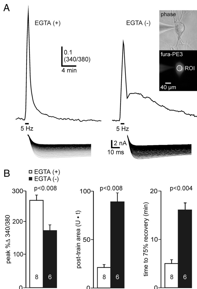
Figure 1. A train of depolarizing stimuli induces a secondary \text{Ca}^{2+} rise sensitive to the \text{Ca}^{2+} chelator, EGTA. A , Simultaneous measurement of free intracellular \text{Ca}^{2+} and membrane current in cultured bag cell neurons using 340/380 fura PE3 fluorescence and whole-cell voltage clamp at -80 mV. A , Inset, A phase contrast image shows the recording pipette, bag cell neuron soma, and its neuritic processes. The bottom image shows the same neuron loaded with fura and the somatic region of interest (ROI) used for data collection. Scale bar applies to both images. A , Top left, \text{Ca}^{2+} influx indicated by a change in intensity of the 340/380 fluorescence ratio following a 1 min, 5 Hz train of 75 ms steps from -80 to 0 mV. With 5 mM intracellular EGTA, stimulation causes a large rise in \text{Ca}^{2+} followed by a rapid recovery to the prestimulus baseline. Top right, In the absence of intracellular EGTA, there is a prolonged \text{Ca}^{2+} plateau subsequent to the initial influx that greatly outlasts the stimulus duration, indicative of CICR. A , Bottom, Traces depict 300 overlaid \text{Ca}^{2+} currents from each pulse to 0 mV of the 1 min train stimulus in either 5 or 0 mM intracellular EGTA. The shifting band of traces is due to use-dependent inactivation of \text{Ca}^{2+} currents during the train stimulus. Unless stated otherwise, all cells were recorded in a \text{Cs}^+ -external and TEA-external (to replace \text{K}^+ and \text{Na}^+ , respectively) and a \text{Cs}^+ -based intracellular solution (to replace intracellular \text{K}^+ ). B , Left, The percentage change in 340/380 from baseline to the peak response during the train stimulus is significantly larger in 5 mM EGTA versus 0 mM EGTA (unpaired Student's t test). For this and subsequent bar graphs, data represents the mean \pm SE, and the n -value is indicated within the bars. B , Middle and right, Zero mM EGTA significantly increases the total area measured from 1 min after stimulation to 11 min post-train stimulus (Mann–Whitney U test) and the time to reach 75% recovery to baseline \text{Ca}^{2+} from the peak of the plateau (Mann–Whitney U test).
