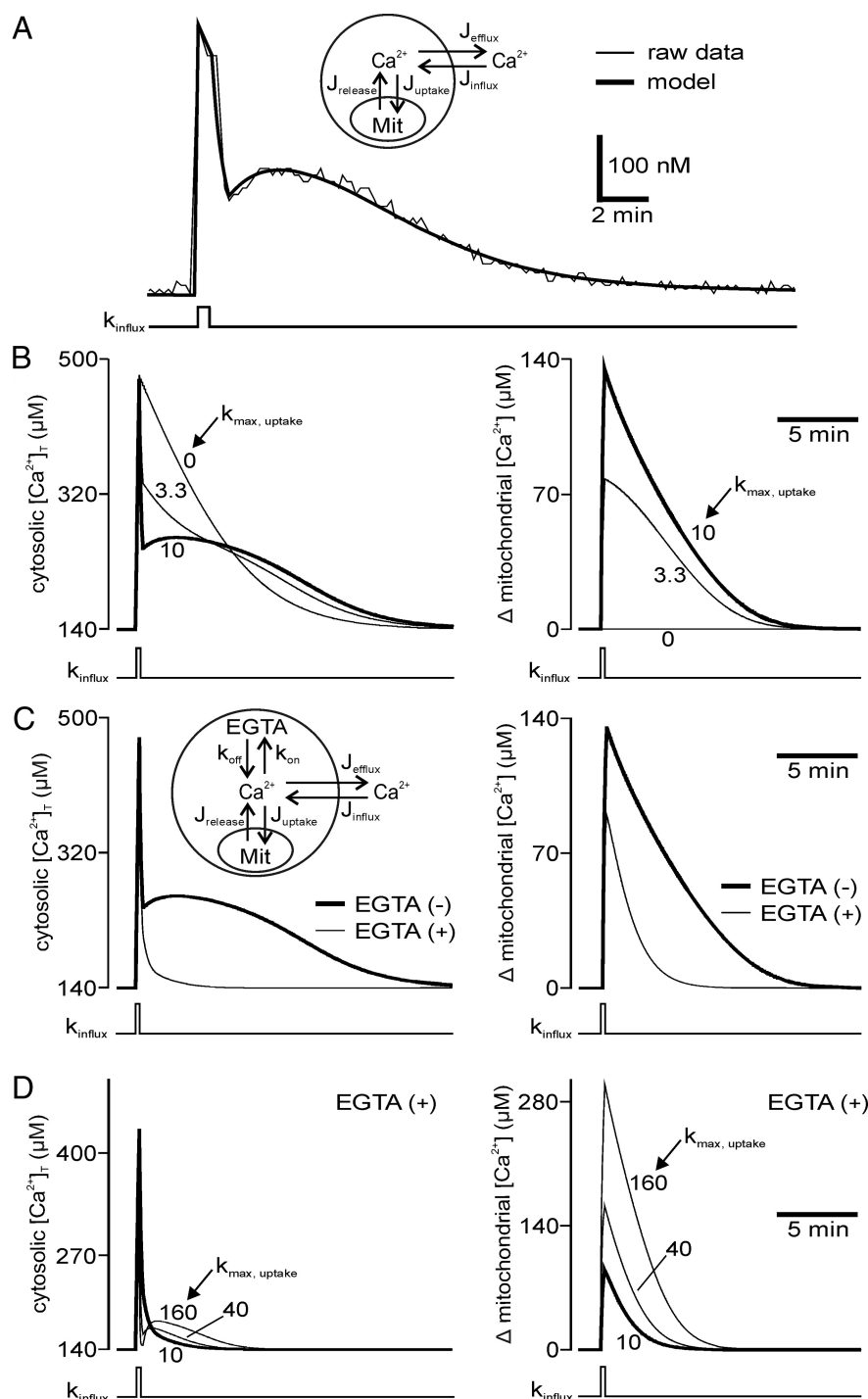
Figure 7. A model of bag cell neuron \text{Ca}^{2+} dynamics demonstrates the sensitivity of mitochondrial \text{Ca}^{2+} release to the \text{Ca}^{2+} chelating agent, EGTA. A , The inset illustrates the components involved in the 3 compartment model of \text{Ca}^{2+} . \text{Ca}^{2+} influx is represented by J_{\text{influx}} , cytosolic \text{Ca}^{2+} removal is mediated by mitochondrial uptake ( J_{\text{uptake}} ) or plasma membrane efflux ( J_{\text{efflux}} ), and mitochondrial \text{Ca}^{2+} release is denoted as J_{\text{release}} . Collectively, these variables determine the cytosolic and mitochondrial \text{Ca}^{2+} concentrations (see Materials and Methods). Raw data from a bag cell neuron (light trace) presenting stimulus-induced \text{Ca}^{2+} influx, CICR, and recovery is fit by the model (dark trace) to estimate values for free intracellular \text{Ca}^{2+} fluxes. Train stimulus-induced \text{Ca}^{2+} influx (bottom) is simulated in the model by transiently increasing the \text{Ca}^{2+} influx rate constant ( k_{\text{influx}} ). Directly after reducing k_{\text{influx}} there is a rapid recovery leading to a prolonged \text{Ca}^{2+} plateau that readily fits the raw data (root mean square error: 2.3 \times 10^{-8} ). Parameters for this fit are ( \pm 95\% confidence interval): V_{\text{max, efflux}} : 6.2 \pm 0.26 \text{ nm/s} , k_{\text{max, uptake}} : 4.45 \pm 0.82 \text{ (s}^{-1}\text{)} , V_{\text{max, release}} : 6.2 \pm 1.14 \text{ nm/s} . Unless otherwise stated, all subsequent model presentations were derived using the average values presented in Table 1. The values in Table 1 reflect parameters measured from changes to free \text{Ca}^{2+} , before converting to rates of total \text{Ca}^{2+} . B , For this and subsequent model graphs, \text{Ca}^{2+} levels reflect total, rather than free intracellular \text{Ca}^{2+} to correct for the presence of exogenous (fura and/or EGTA) and endogenous \text{Ca}^{2+} buffers present when estimating rates (see Materials and Methods). Serially reducing the rate constant of mitochondrial \text{Ca}^{2+} uptake ( k_{\text{max, uptake}} ) from 10 to 3.3 then 0 ( \text{s}^{-1} )
