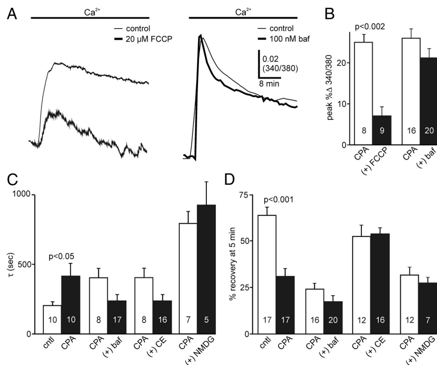
Figure 9. Store-operated \text{Ca}^{2+} influx is reduced in magnitude by FCCP but is not influenced by acidic stores, the PMCA, or the \text{Na}^+/\text{Ca}^{2+} exchanger. A , Left, Neurons exposed to 20 \mu\text{M} FCCP before the addition of extracellular \text{Ca}^{2+} (dark trace) causes a reduction in store-operated influx relative to control (light trace). A , Right, Exposure to 100 \text{ nM} bafilomycin A (baf) before the addition of extracellular \text{Ca}^{2+} (dark trace) does not influence the size or recovery of store-operated \text{Ca}^{2+} influx. Neurons were previously depleted in \text{Ca}^{2+} -free ASW with 20 \mu\text{M} CPA. B , Treatment with FCCP significantly reduces the peak \text{Ca}^{2+} influx after the addition of extracellular \text{Ca}^{2+} (left), whereas bafilomycin has no effect (both comparisons using Mann–Whitney U test). C , Summary data demonstrating that the mean decay time constant ( \tau ) is significantly larger in CPA (Welch corrected unpaired Student's t test), but not in bafilomycin (unpaired Student's t test), 20 \mu\text{M} carboxyeosin (CE) (Welch corrected Student's t test), or where extracellular \text{Na}^+ is replaced with NMDG (Mann–Whitney U test). D , CPA pretreatment significantly reduces the percentage recovery from peak \text{Ca}^{2+} , whereas incubation with bafilomycin, carboxyeosin, or extracellular NMDG does not (all comparisons using unpaired Student's t test).
