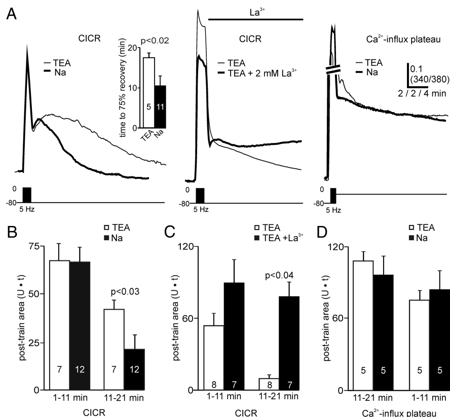
Figure 6. Mitochondrial \text{Ca}^{2+} release is removed by the \text{Na}^+/\text{Ca}^{2+} exchanger and the PMCA. A , Left, In the absence of extracellular \text{Na}^+ (TEA, light trace), the mitochondrial \text{Ca}^{2+} plateau evoked by a 1 min, 5 Hz train stimulus from -80 mV is prolonged compared with cells bathed in extracellular \text{Na}^+ (dark trace). A , Inset, The presence of extracellular \text{Na}^+ significantly accelerated the time to 75% recovery for CICR (Mann–Whitney U test). A , Middle, In \text{Na}^+ -free extracellular saline (TEA), the application of \text{La}^{3+} (dark trace) during the onset of CICR occludes recovery. In these experiments, cells are voltage-clamped at -80 mV following the stimulus. A , Right, As a control, a 1 min 5 Hz train stimulus from -80 mV, followed by a prolonged step depolarization evokes a \text{Ca}^{2+} plateau similar to CICR (at break, a portion of the \text{Ca}^{2+} influx is omitted for clarity to emphasize the \text{Ca}^{2+} plateau). The recovery of this \text{Ca}^{2+} -influx plateau is insensitive to the replacement of extracellular \text{Na}^+ (dark trace) for TEA (light trace). For this experiment, neurons are pretreated with 100 \mu\text{M} TPP to prevent any influence of mitochondrial \text{Ca}^{2+} release and are recorded with 0 \text{ mM} intracellular EGTA. B , The post-train stimulus area from 1 to 11 min during mitochondrial \text{Ca}^{2+} release is not significantly different between \text{Na}^+ and TEA conditions (unpaired Student's t test). However, the area from 11 to 21 min is significantly larger in TEA-containing extracellular saline (Mann–Whitney U test). C , In the absence of \text{Na}^+/\text{Ca}^{2+} exchanger activity, the application of 2 \text{ mM} \text{La}^{3+} during CICR does not alter the post-train stimulus area from 1 to 11 min (Mann–Whitney U test), but significantly increases the area from 11 to 21 min (Welch corrected Student's t test, respectively). D , Area summary data for the \text{Ca}^{2+} plateau evoked by post-train stimulus depolarization at (ranging from -10 to -20 mV). Replacing extracellular \text{Na}^+ with TEA does not significantly alter the post-train stimulus area from time 1–11 min or 11–21 (Student's t test for both).
